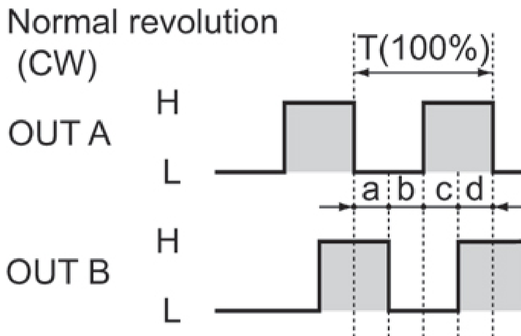
Example of a Pulse Train Output waveform.
