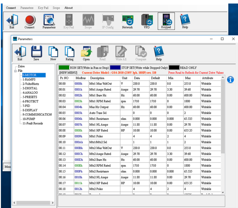
Convenient software tools, including a parameter dialog and scope window.
