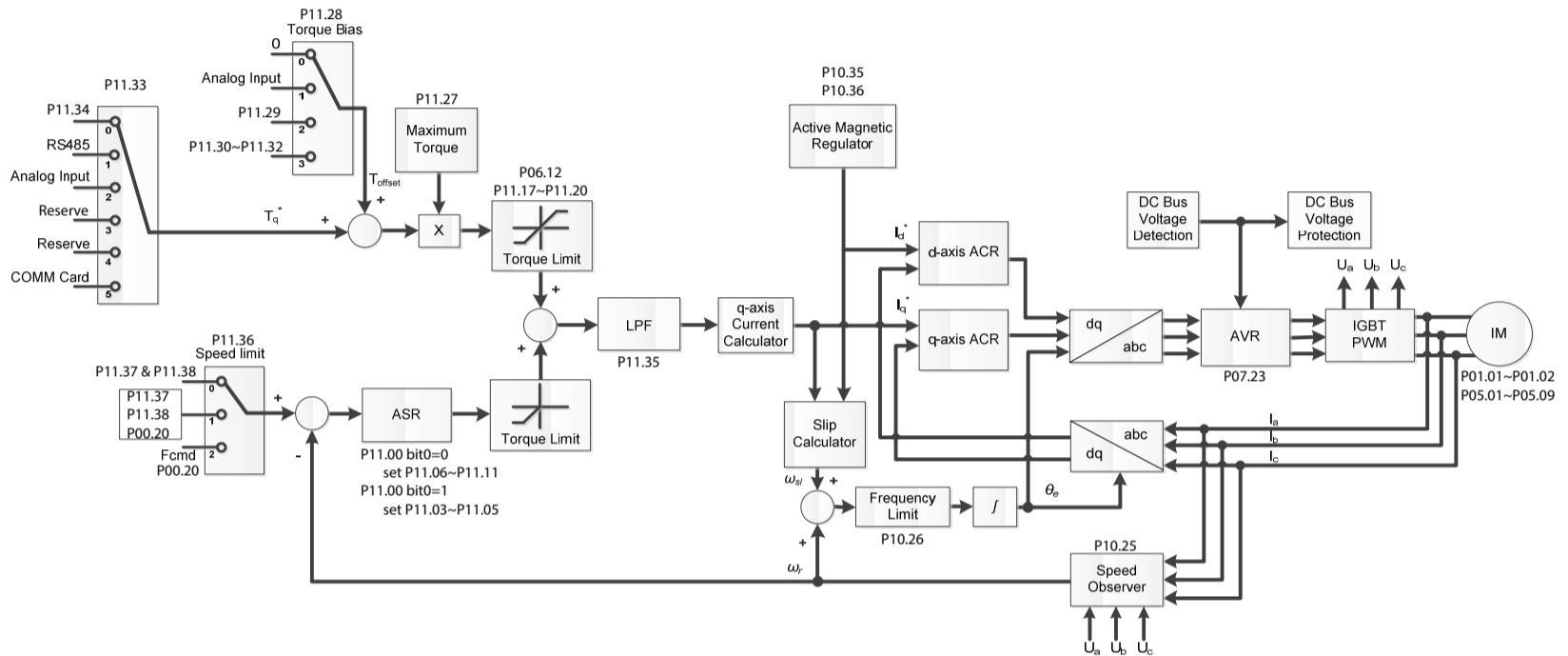
Example of a torque control function block diagram.
