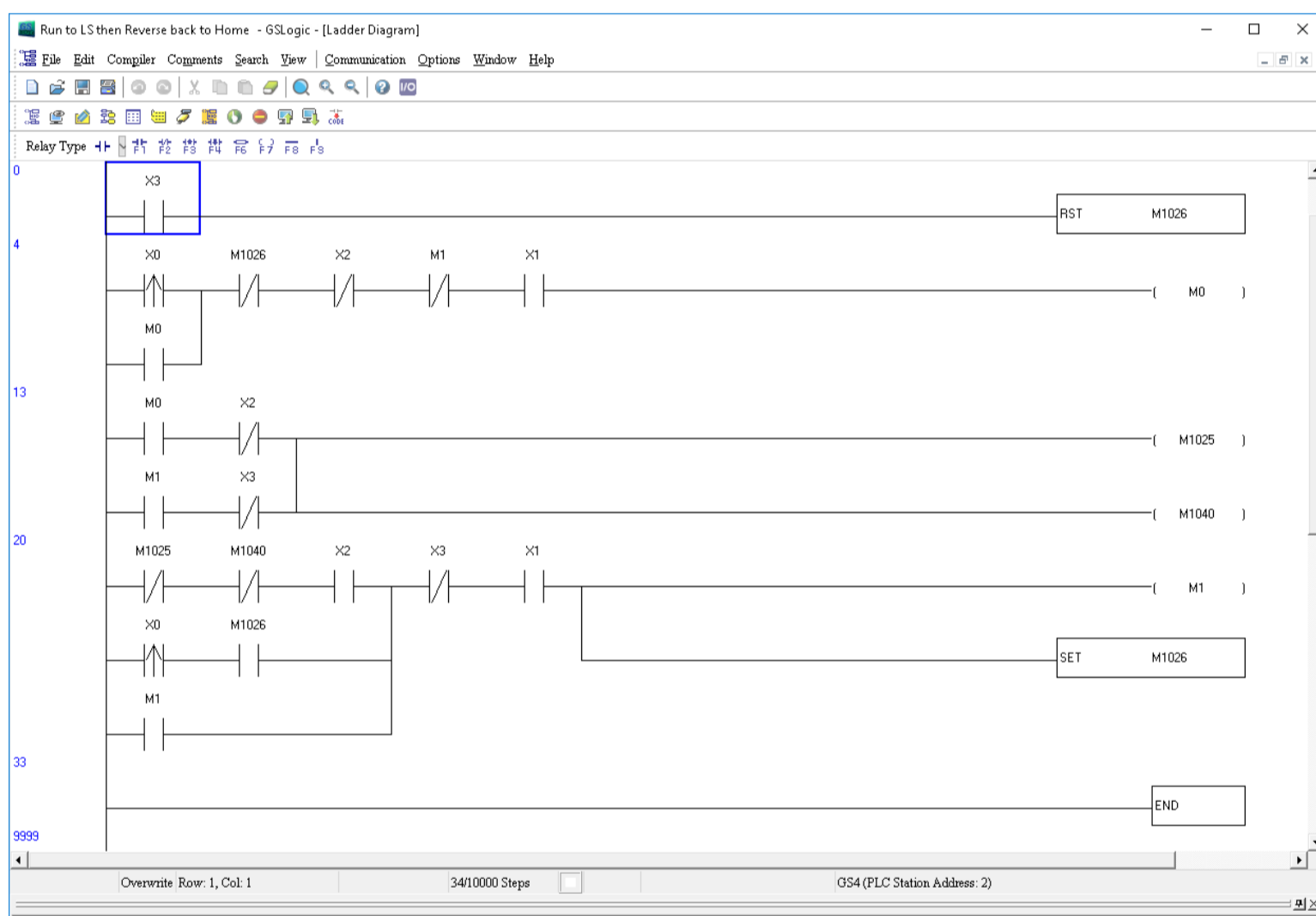
Example of a ladder logic program in the built-in PLC of a VFD.
